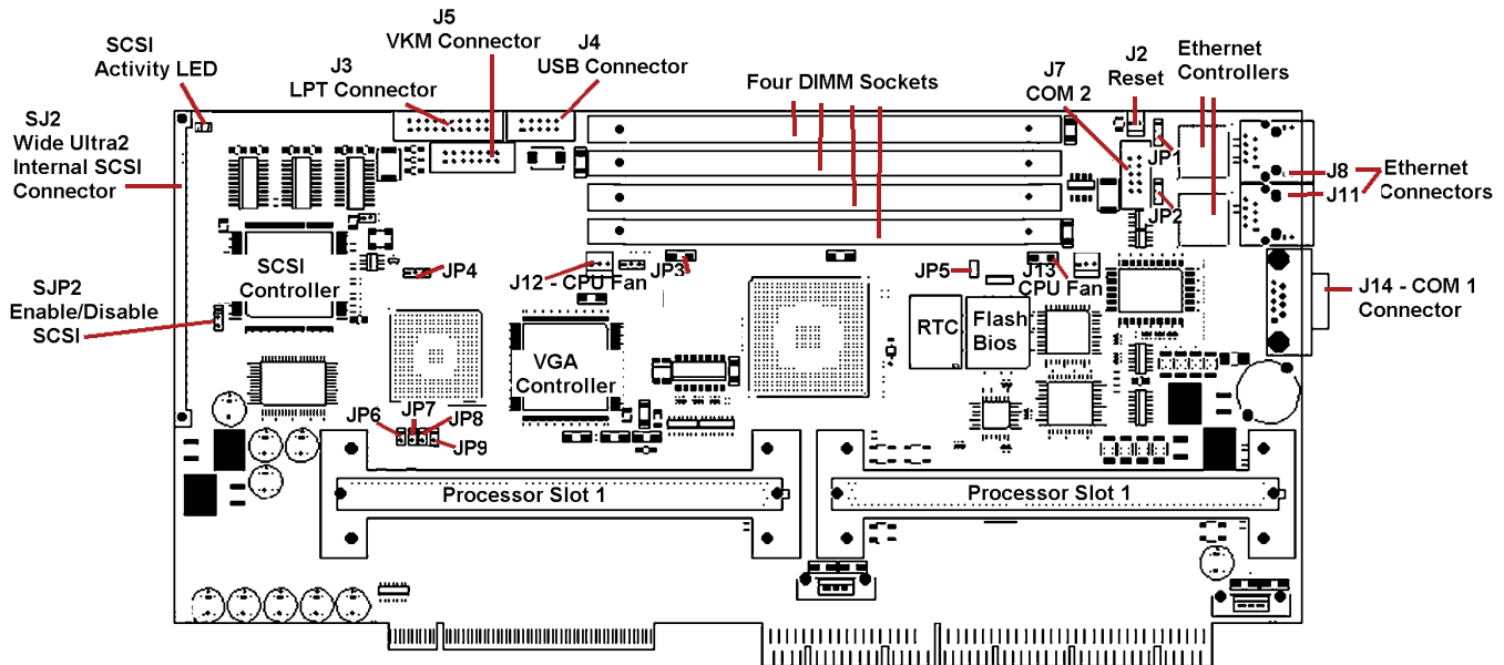
Figure 2 DP8xxx Series Board Layout
