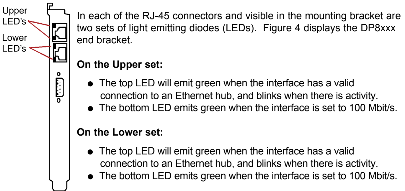
Figure 4 DP8xxx End Bracket
